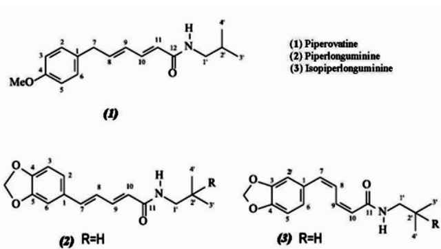
Figure 1. Chemical structures of the isobutylamides of Ottonia martiana .
